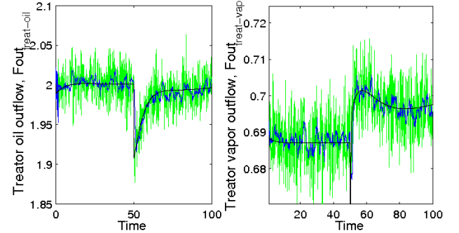
Fig. 5. ANDDR results for a positive setpoint change
