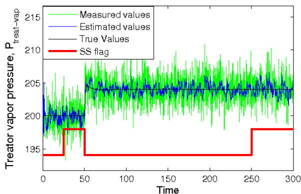
Fig. 7. Hybrid NDDR results solving transition problem for P_{treat-vap}
