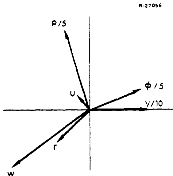
Figure 74. Exact Dutch Roll Eigenvector Diagram Corresponding to Empirical Aerodynamic Data
