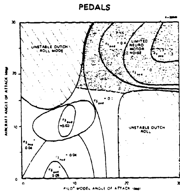
Figure 40b Performance Contours for Single and Dual Controls (ARI On) (Continued)
