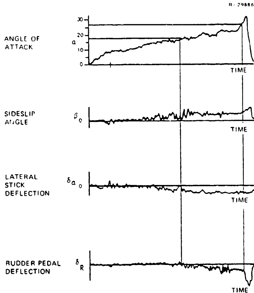
Figure 42 Results of Manned Simulation
