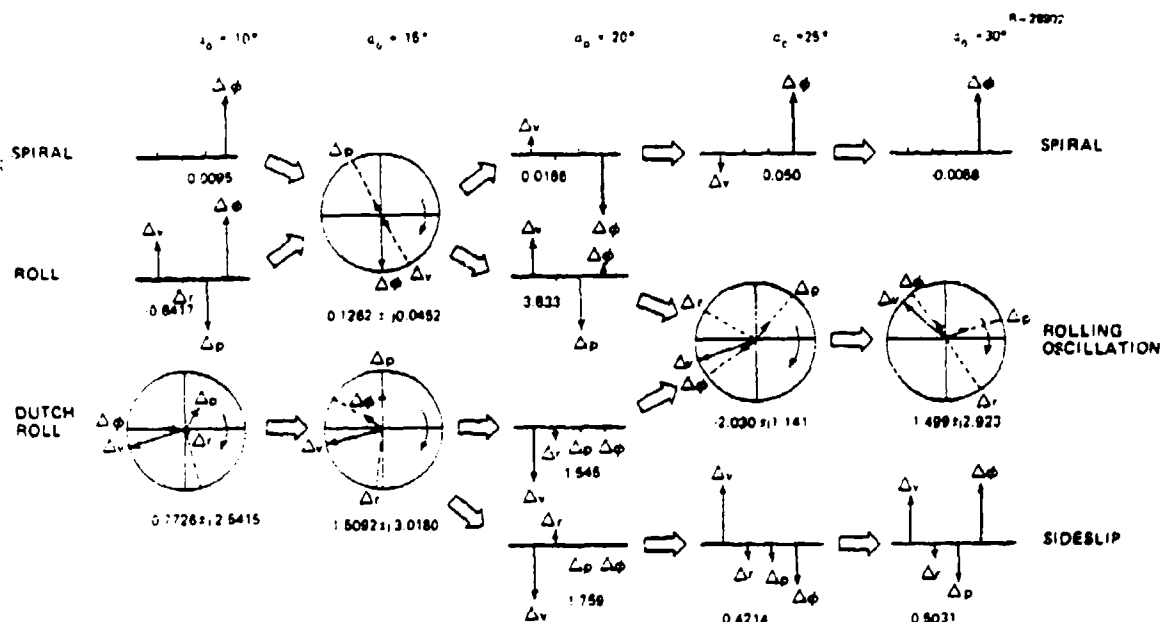
Figure 6 Eigenvector Evolution with Angle of Attack ( M=0.8 )
