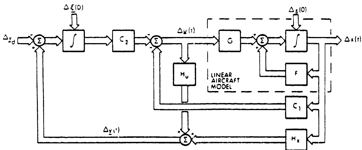
Figure 46 Type 1 DPCAS with Control-Rate Weighting
