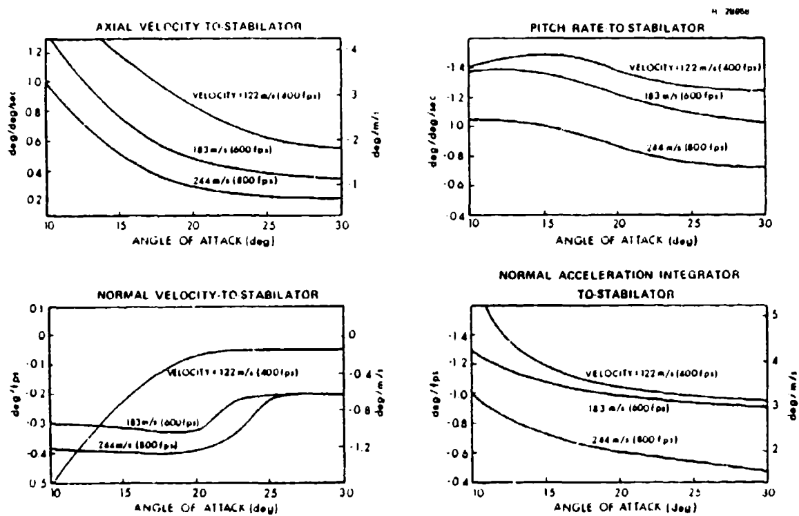
Figure 56 Angle of Attack-Dynamic Pressure Sweep -- Stabilator Type 1 DPCAS Gains
