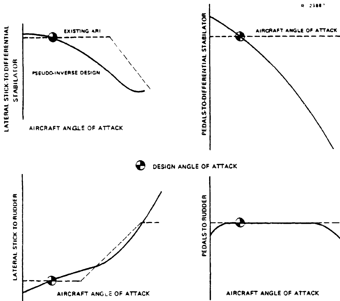
Figure C-1 Comparison of Pseudoinverse ARI Design with Existing ARI Characteristics
