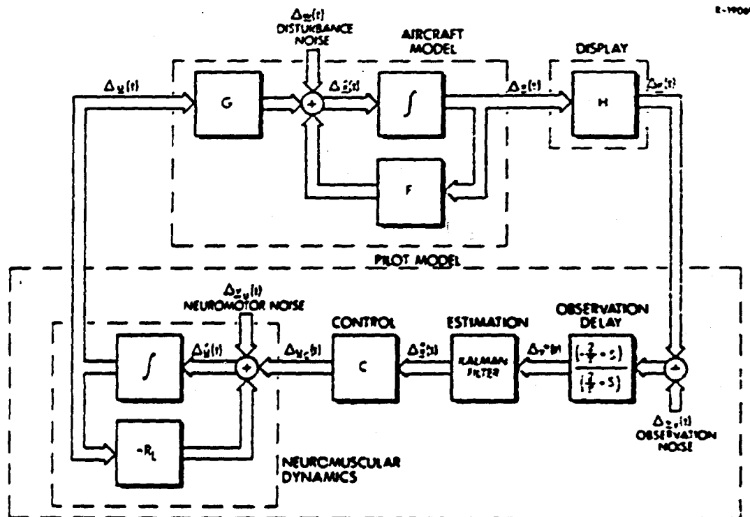
Figure 34 Block Diagram of the Pilot Model Containing the Padé Approximation to Pure Time Delay
