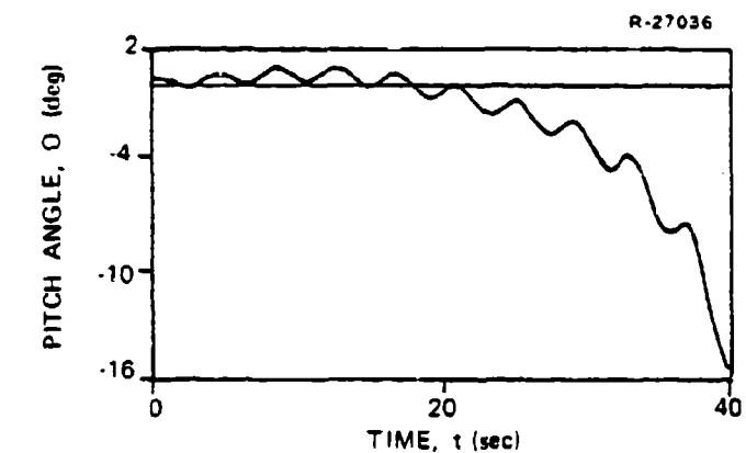
(a) PITCH ANGLE TIME HISTORY
