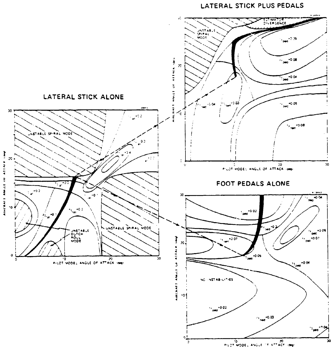
Figure 41 Prediction of Pilot Behavior at High Angle of Attack Under Minimum Control Effort (MCE) Adaptive Behavior Assumption
