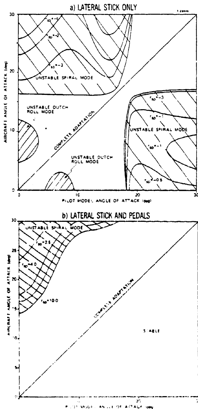
Figure 38 Effects of Pilot Model Adaptation on Maneuvering Flight Stability (ARI Off)
