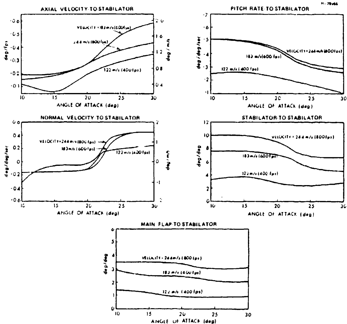
Figure 55 Angle of Attack-Dynamic Pressure Sweep -- Stabilator Type 0 DPCAS Gains
