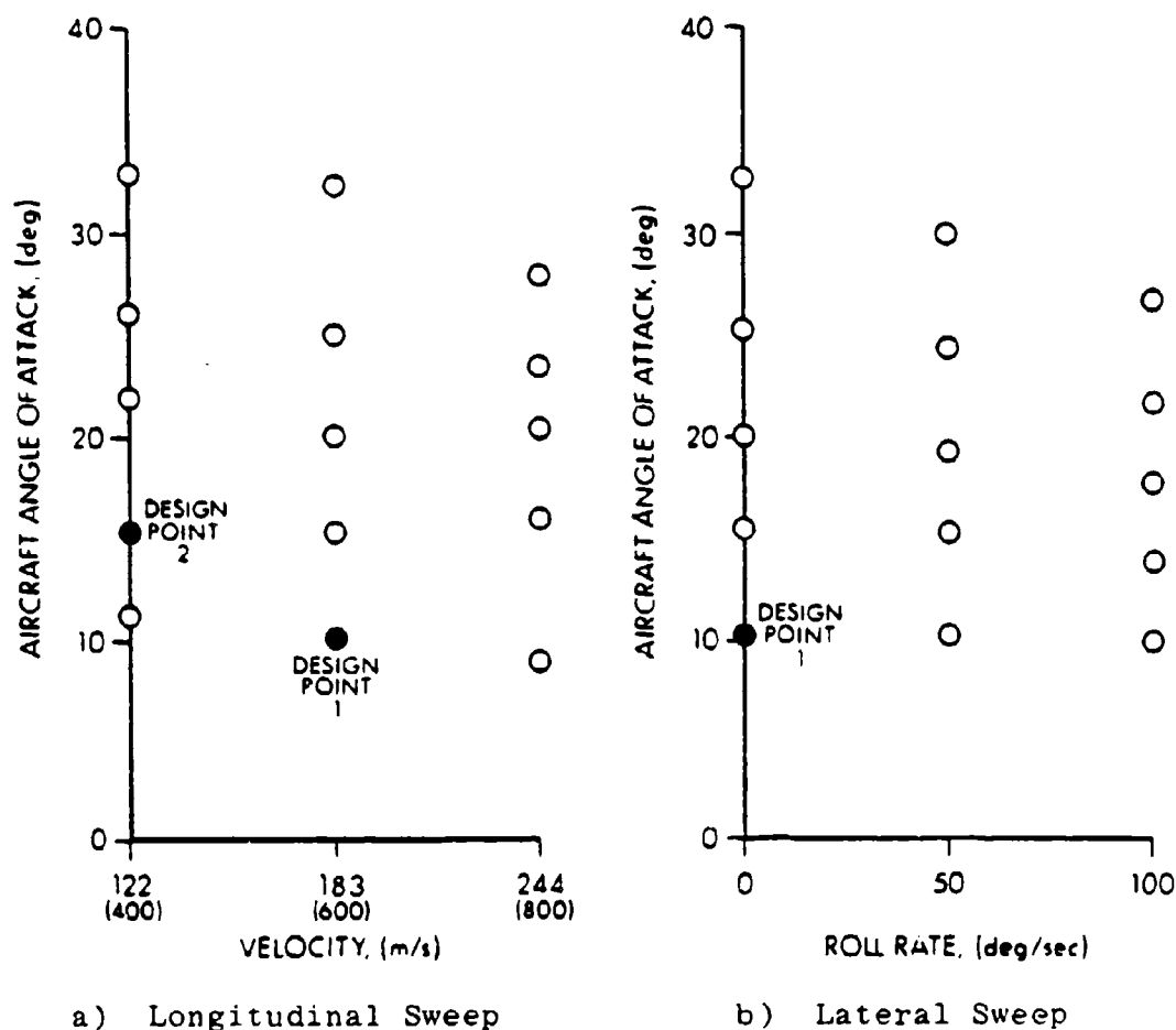
Figure 47 Flight Conditions for DPCAS Point Design
