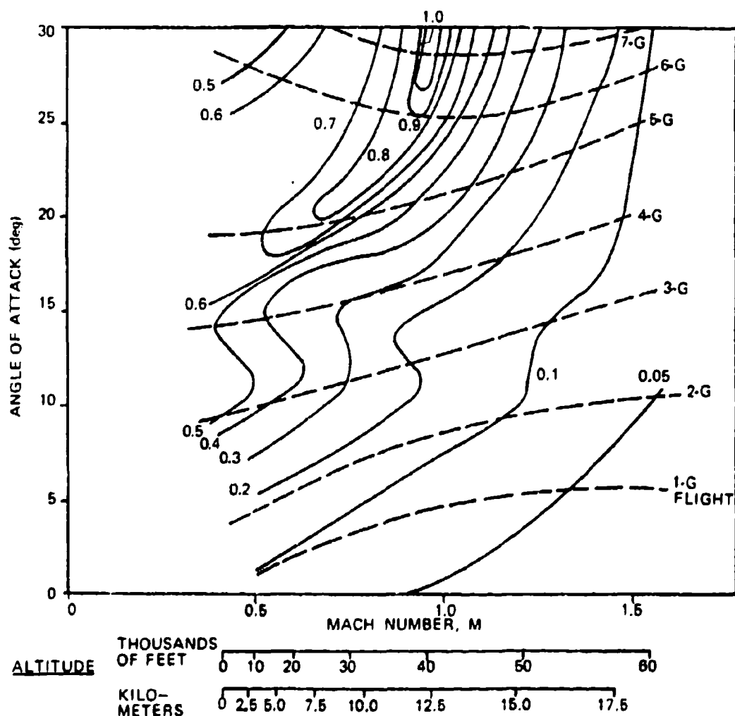
Figure 19 Effects of Compressibility on Dutch Roll Damping Ratio at Constant Dynamic Pressure (q_{\infty} = 11.9 \times 10^3 \text{ Nm}^{-2} (248 \text{ psf}))
