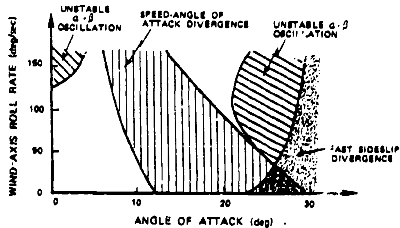
b) TRANSONIC ( M = 0.95 )
