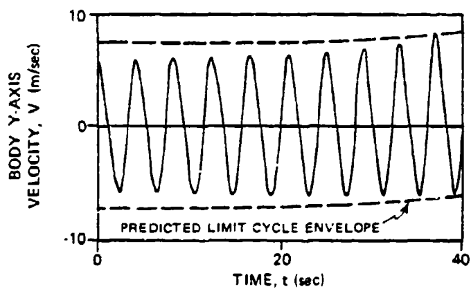
(b) BODY Y-AXIS VELOCITY TIME HISTORY
