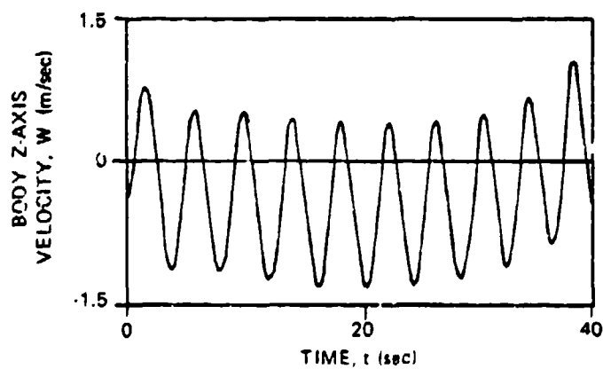
(c) BODY Z-AXIS VELOCITY TIME HISTORY
