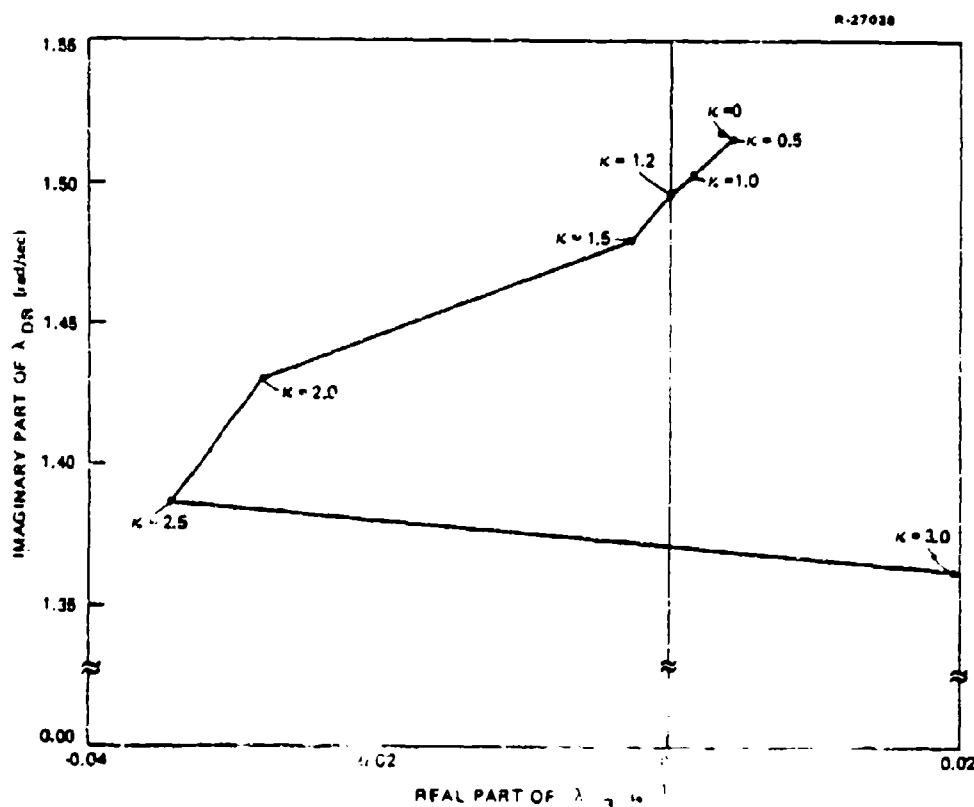
Figure 71 Variation of the Dutch Roll Mode with Assumed Oscillation Amplitude
