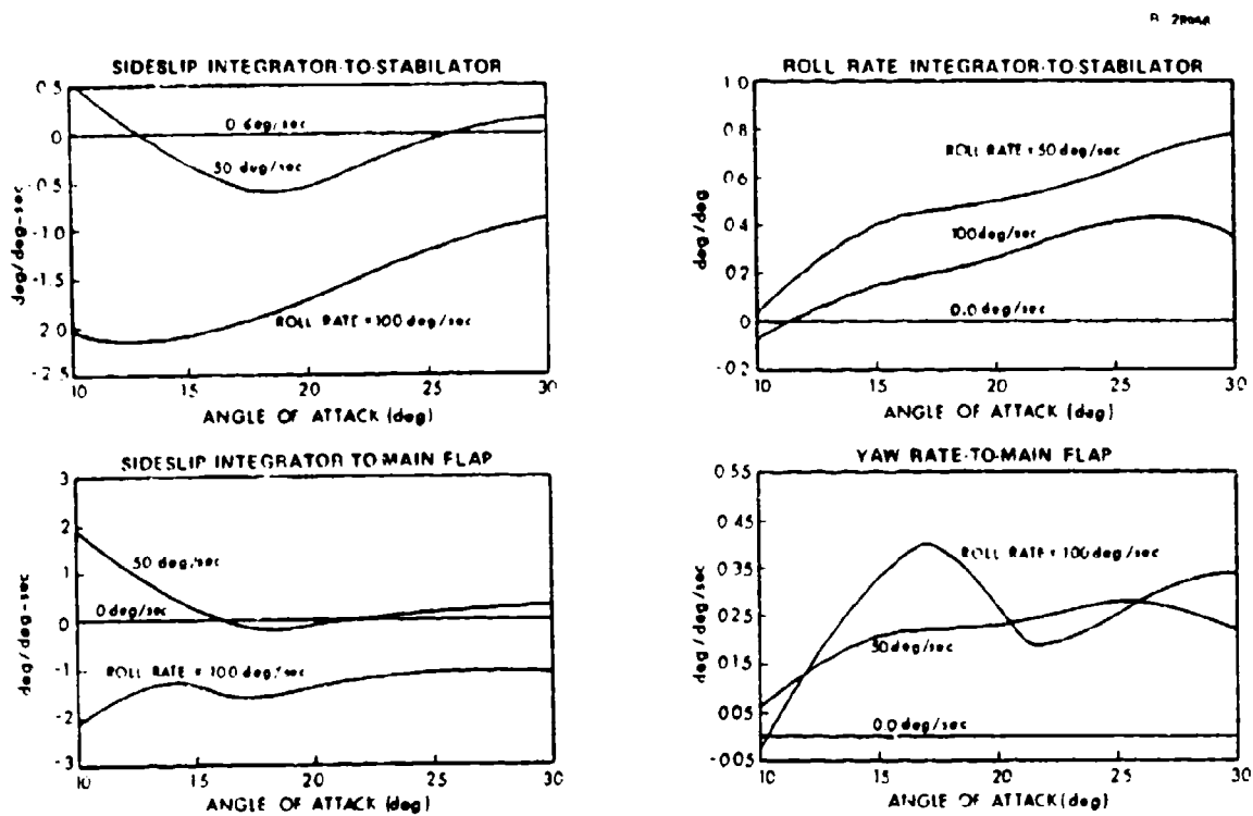
Figure 66 Selected Longitudinal Crossfeed Gains for the Lateral Sweep
