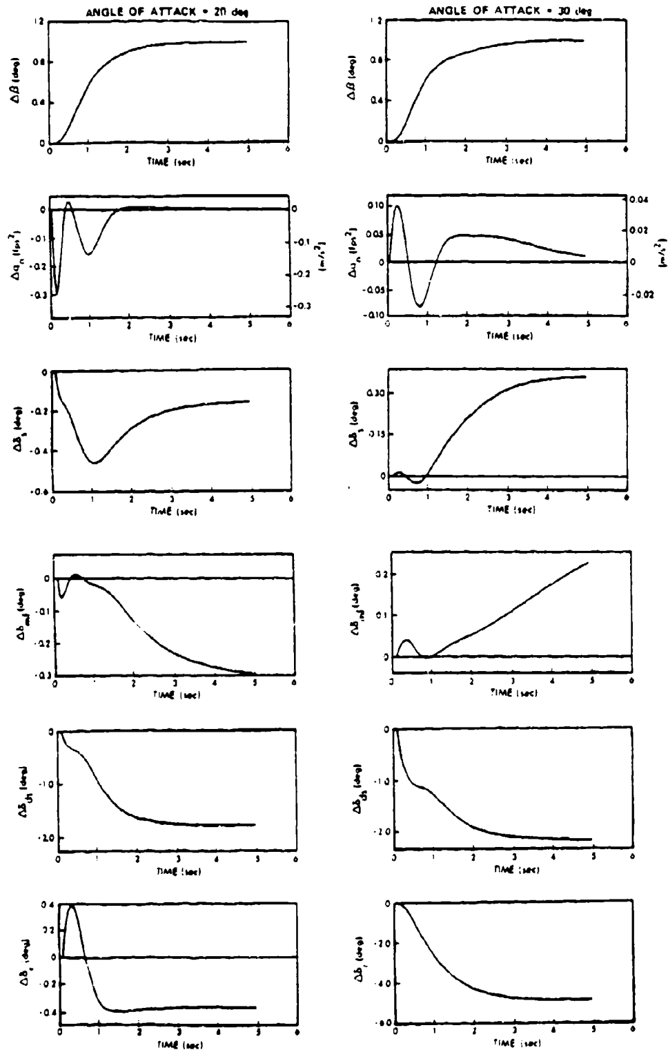
Figure 65 Sideslip Step Responses for Varying Angle of Attack at Constant Roll Rate and Velocity, \Delta \phi_d = 1.0 deg/sec, p_{w_0} = 50 deg/sec, V_0 = 183 m/s
